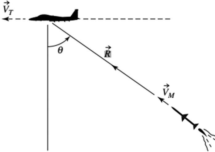
Figure 3. Deviated pursuit guidance. [1: 186]
